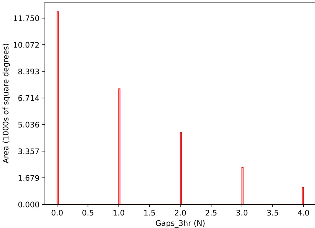
ddf_loaded_half_fl2_v3.4_10yrs i band: Gaps_3hr
