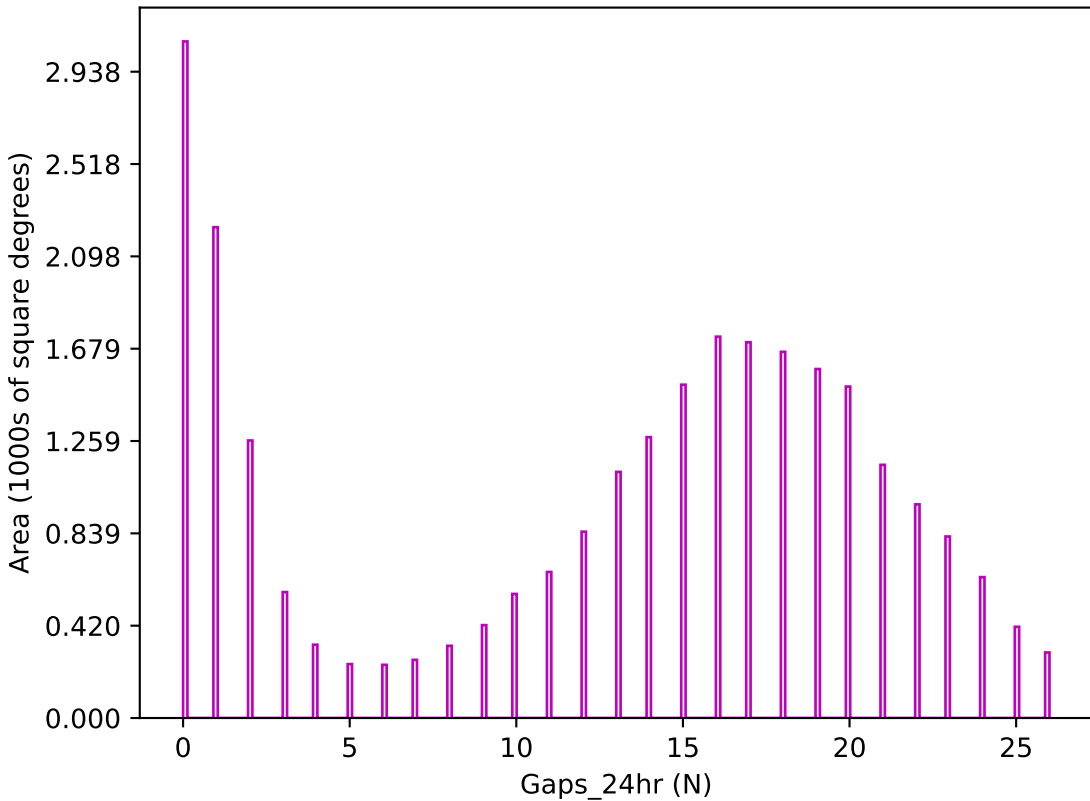
ddf_loaded_half_fl2_v3.4_10yrs z band: Gaps_24hr
