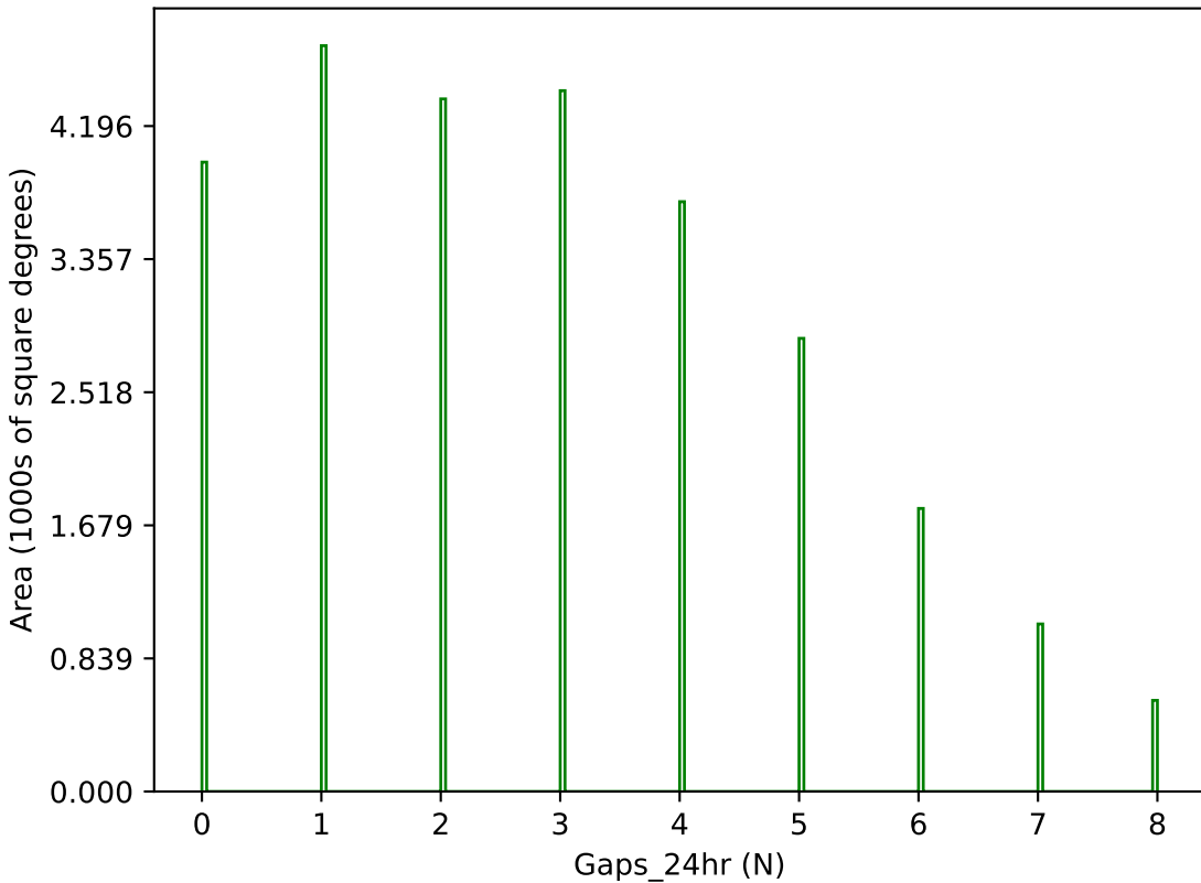
ddf_loaded_half_fl2_v3.4_10yrs g band: Gaps_24hr
