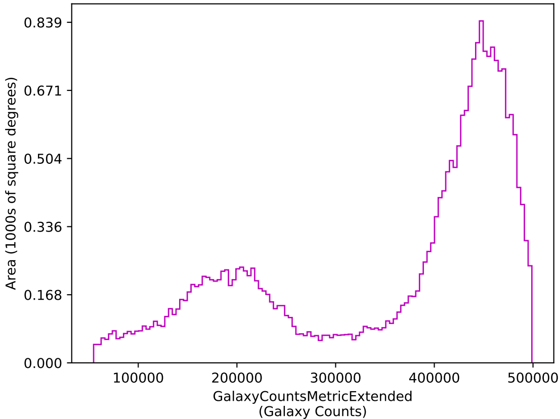
ddf_loaded_half_fl2_v3.4_10yrs z: GalaxyCountsMetricExtended
