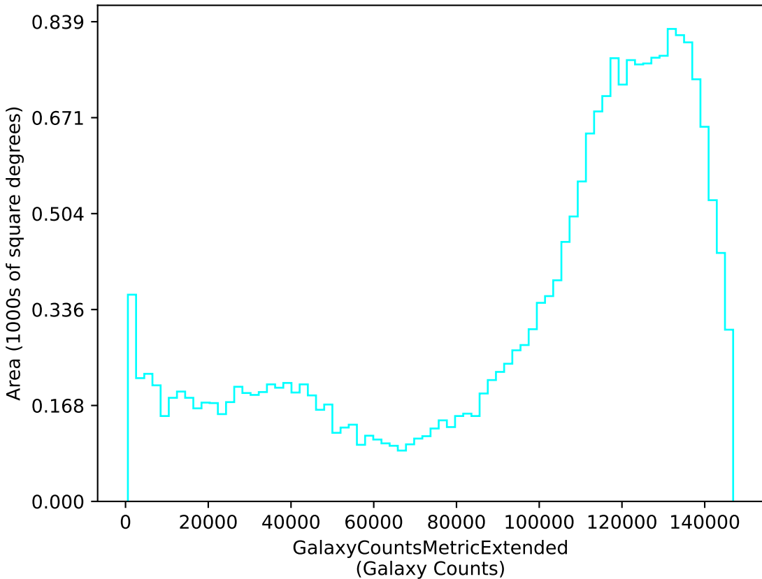
ddf_loaded_half_fl2_v3.4_10yrs u: GalaxyCountsMetricExtended
