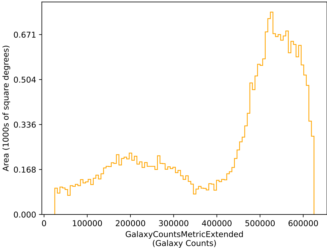
ddf_loaded_half_fl2_v3.4_10yrs r: GalaxyCountsMetricExtended
