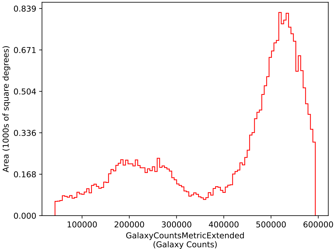
ddf_loaded_half_fl2_v3.4_10yrs i: GalaxyCountsMetricExtended
