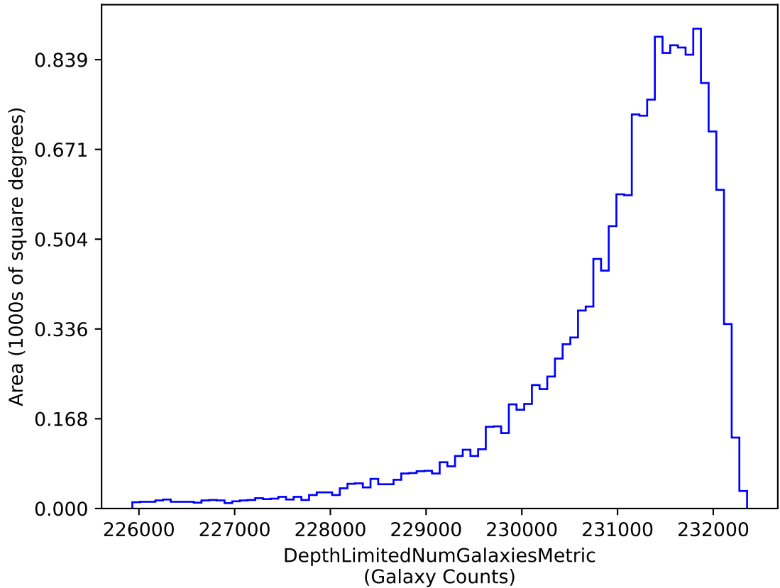
ddf_loaded_half_fl2_v3.4_10yrs i band galaxies non-DD: DepthLimitedNumGalaxiesMetric
