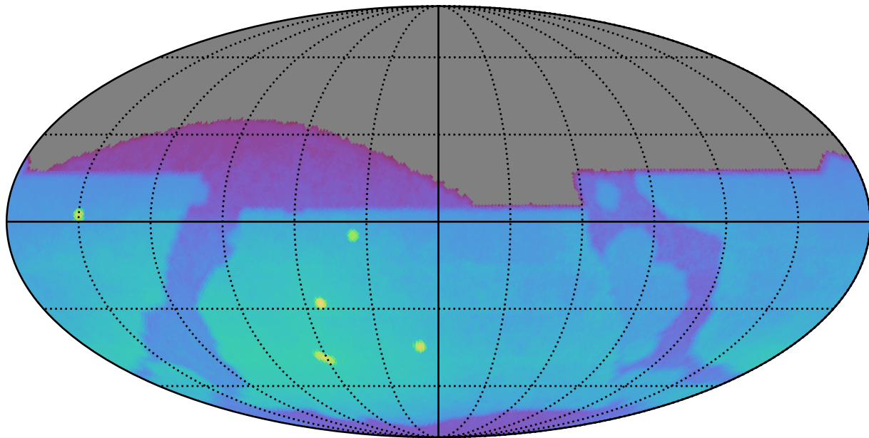
ddf_loaded_half_fl2_v3.4_10yrs : Brown Dwarf, L7
