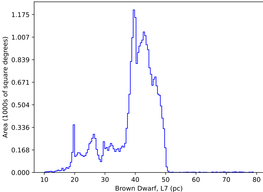
ddf_loaded_half_fl2_v3.4_10yrs : Brown Dwarf, L7
