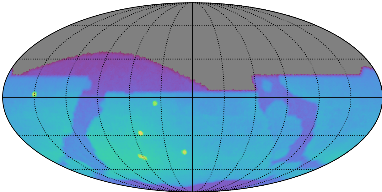
ddf_loaded_half_fl2_v3.4_10yrs : Brown Dwarf, L4
