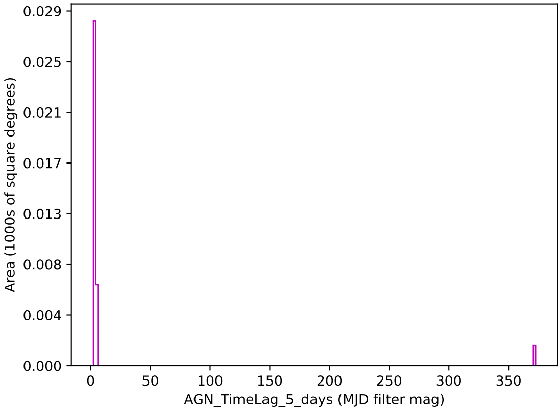
ddf_loaded_half_fl2_v3.4_10yrs z band: AGN_TimeLag_5_days
