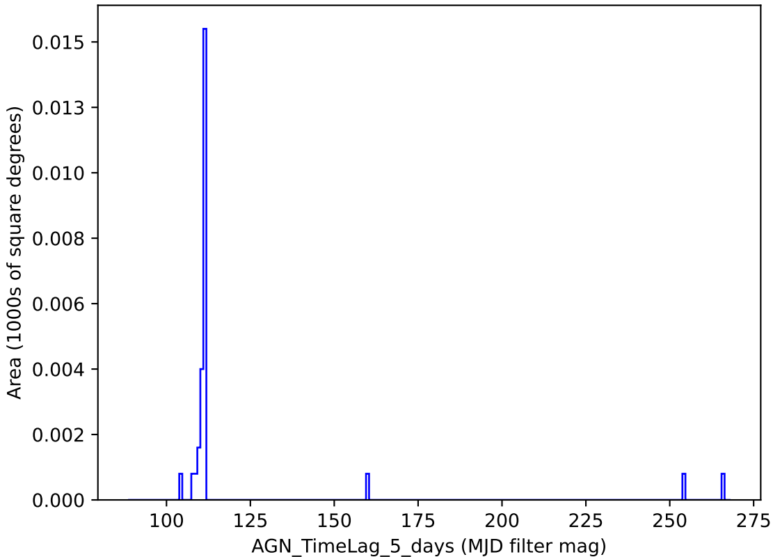
ddf_loaded_half_fl2_v3.4_10yrs y band: AGN_TimeLag_5_days
