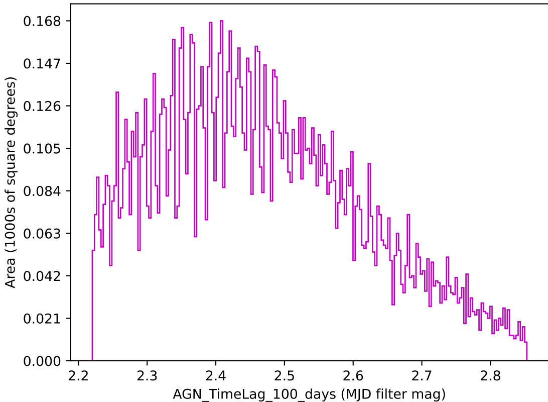
ddf_loaded_half_fl2_v3.4_10yrs z band: AGN_TimeLag_100_days
