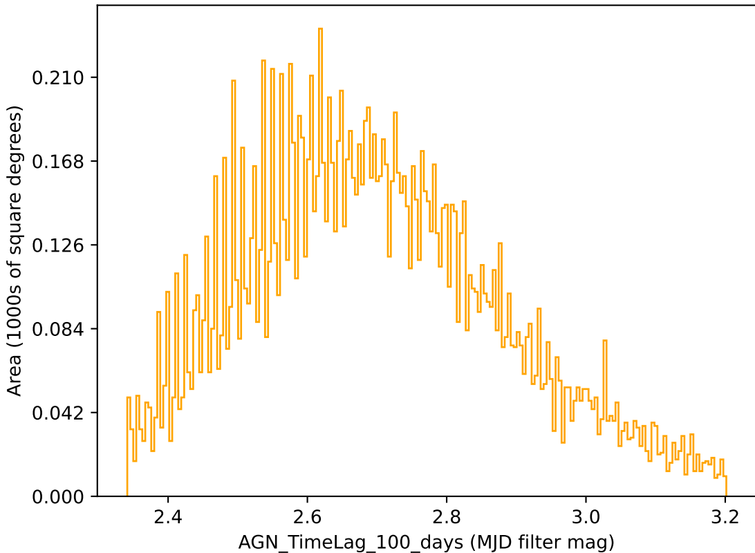
ddf_loaded_half_fl2_v3.4_10yrs r band: AGN_TimeLag_100_days
