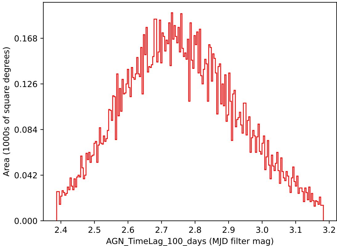
ddf_loaded_half_fl2_v3.4_10yrs i band: AGN_TimeLag_100_days
