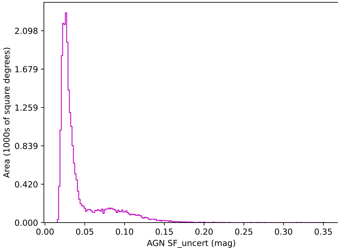
ddf_loaded_half_fl2_v3.4_10yrs z band: AGN SF_uncert
