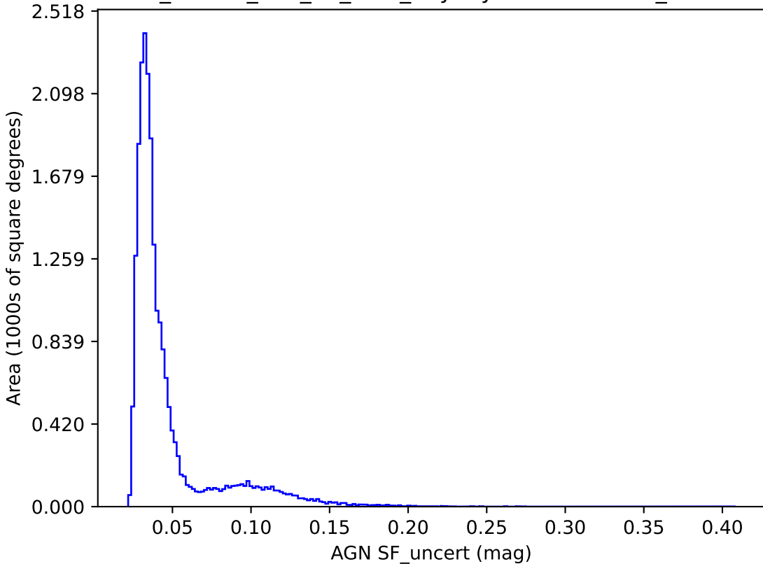
ddf_loaded_half_fl2_v3.4_10yrs y band: AGN SF_uncert
