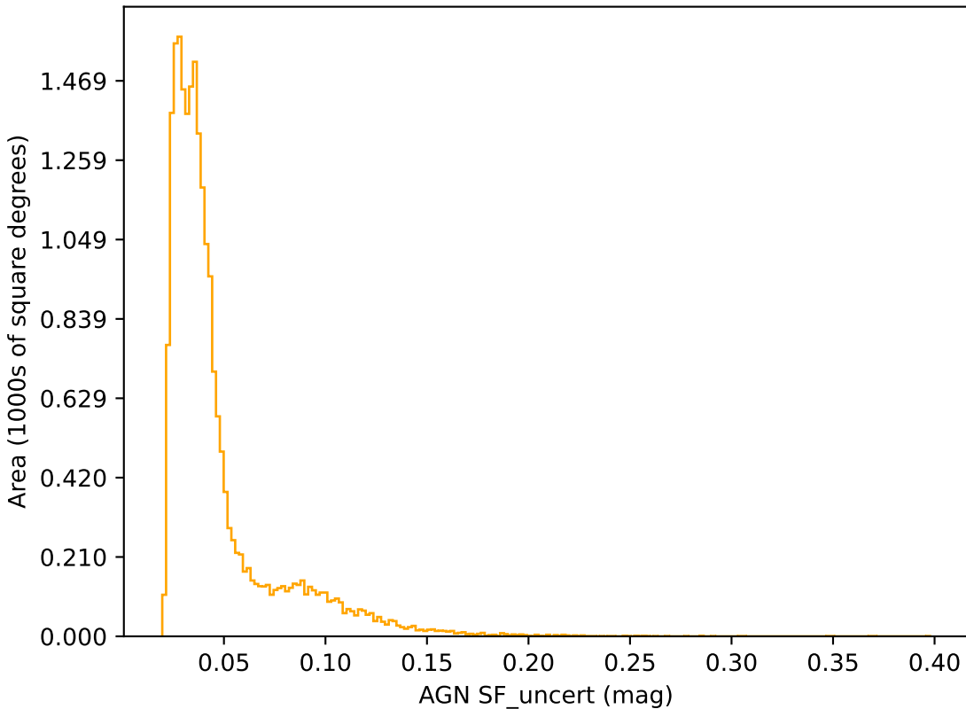
ddf_loaded_half_fl2_v3.4_10yrs r band: AGN SF_uncert
