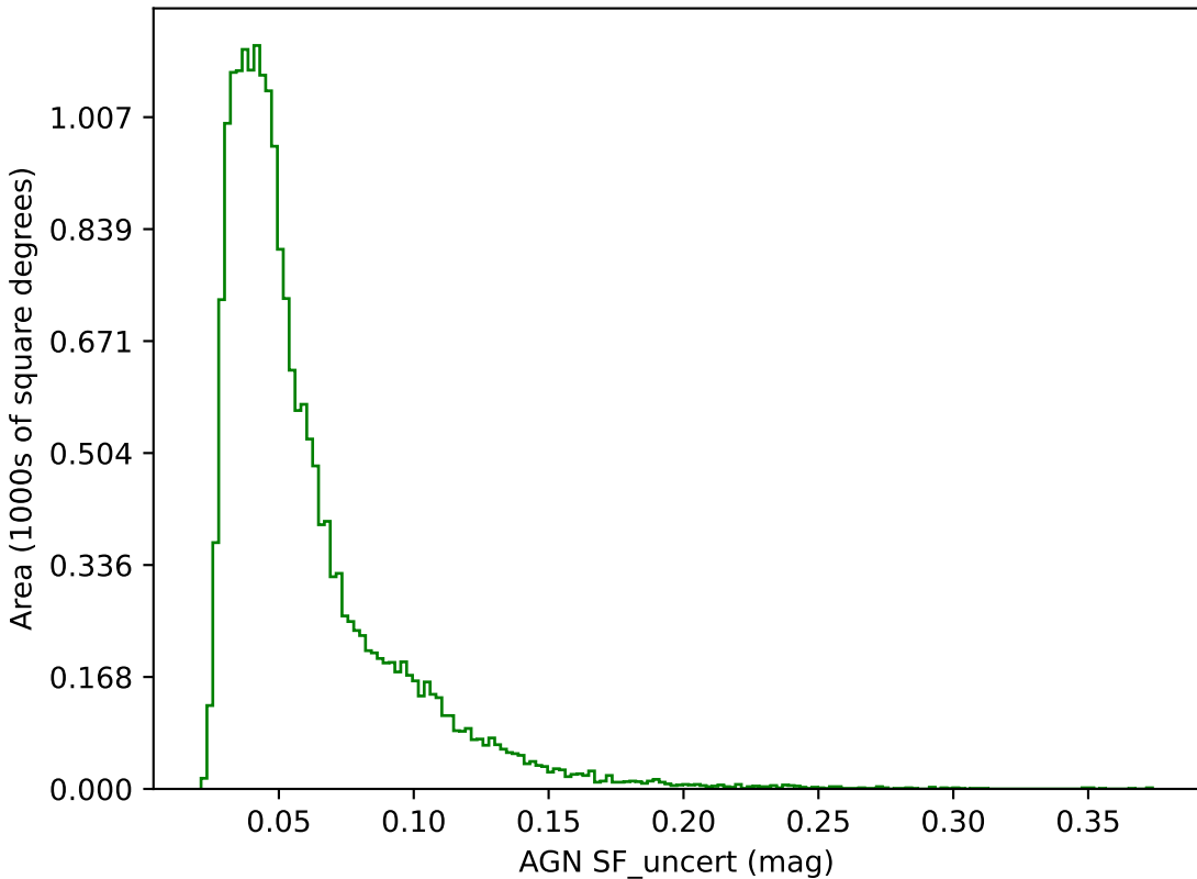
ddf_loaded_half_fl2_v3.4_10yrs g band: AGN SF_uncert
