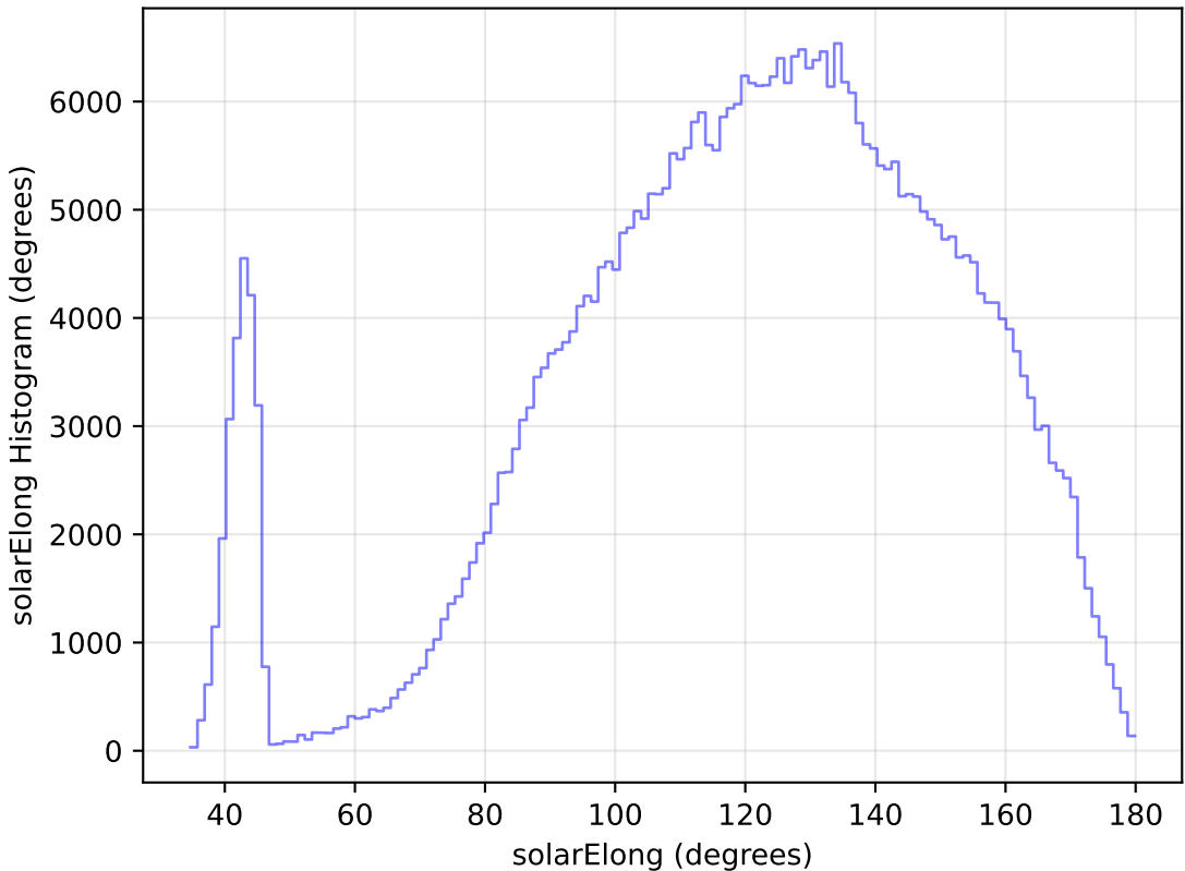
ddf_loaded_half_fl2_v3.4_10yrs WFD z band: solarElong Histogram
