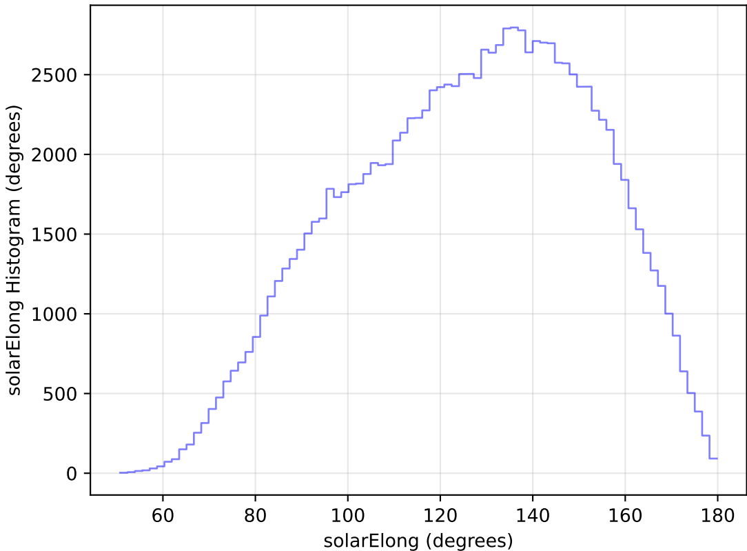
ddf_loaded_half_fl2_v3.4_10yrs WFD u band: solarElong Histogram
