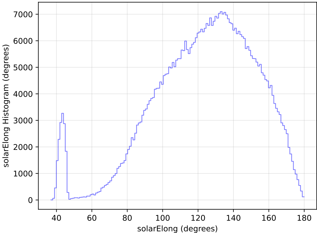
ddf_loaded_half_fl2_v3.4_10yrs WFD r band: solarElong Histogram
