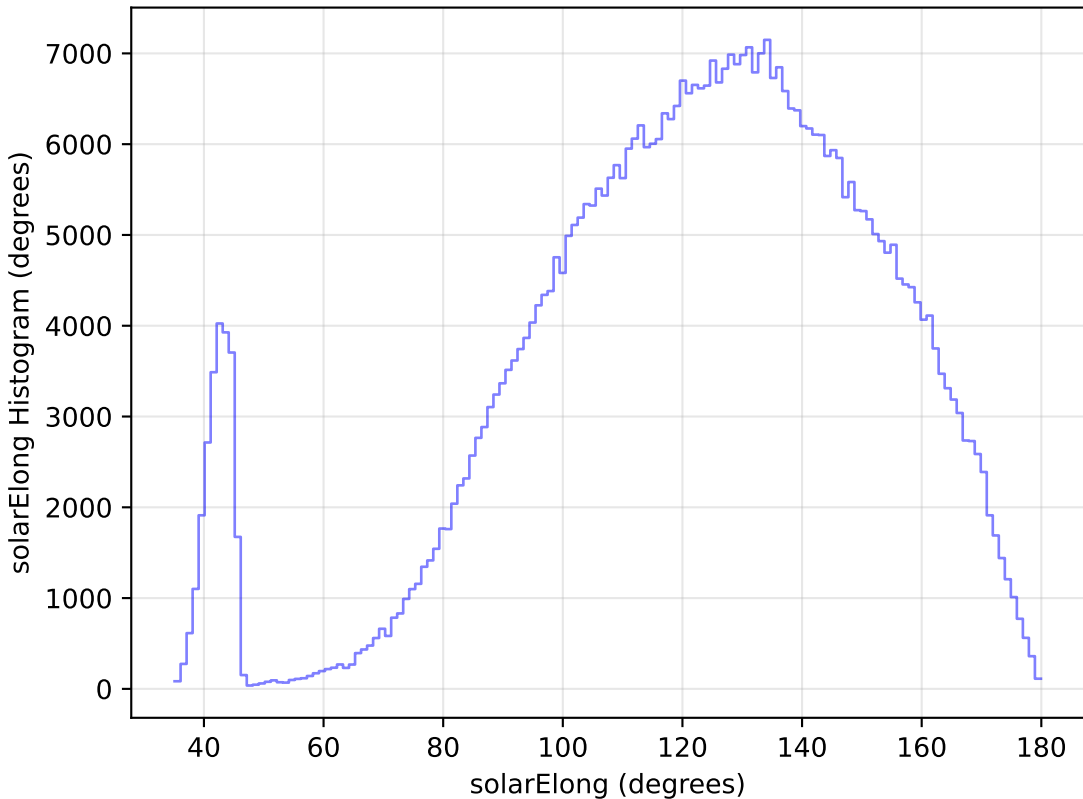
ddf_loaded_half_fl2_v3.4_10yrs WFD i band: solarElong Histogram
