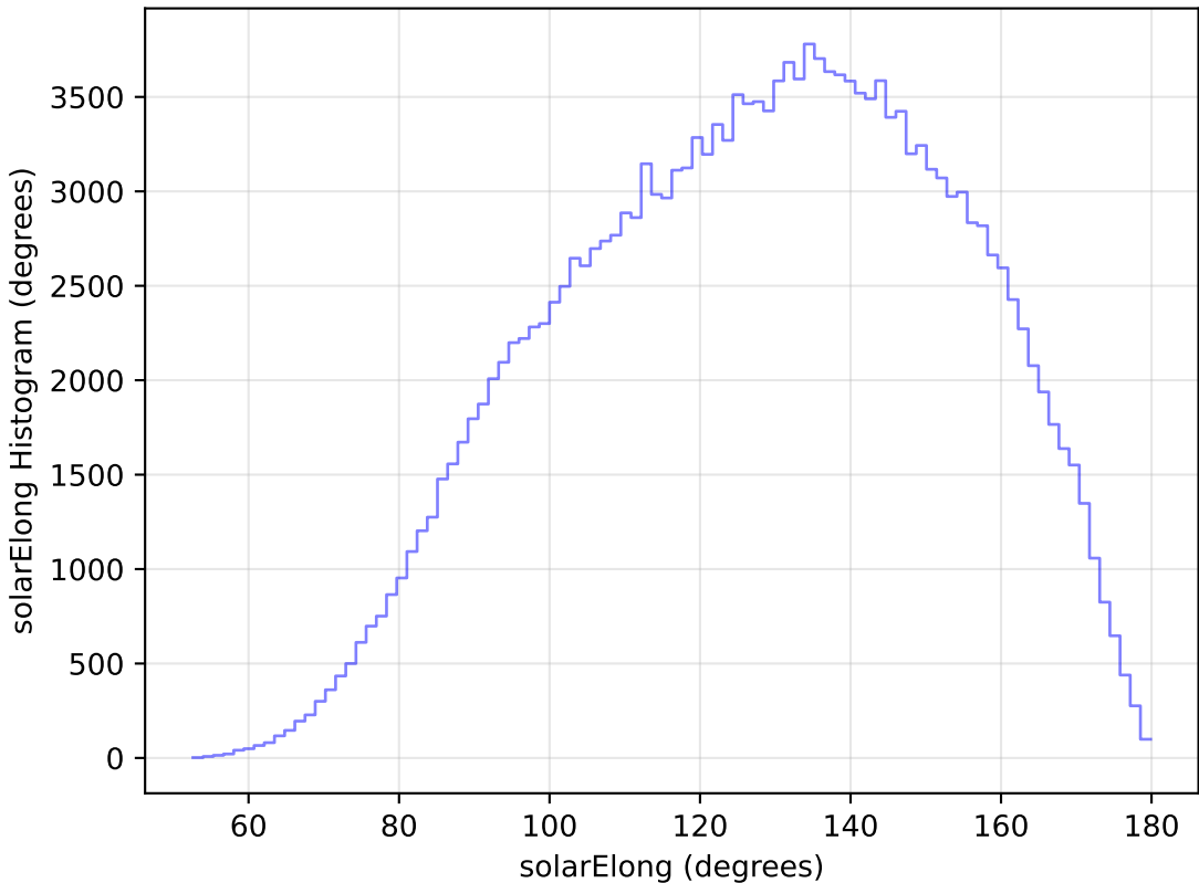
ddf_loaded_half_fl2_v3.4_10yrs WFD g band: solarElong Histogram
