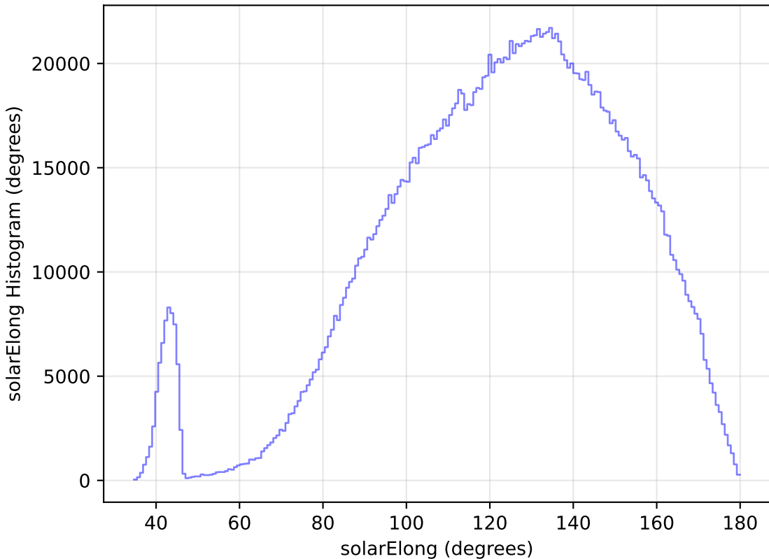
ddf_loaded_half_fl2_v3.4_10yrs WFD all bands: solarElong Histogram
