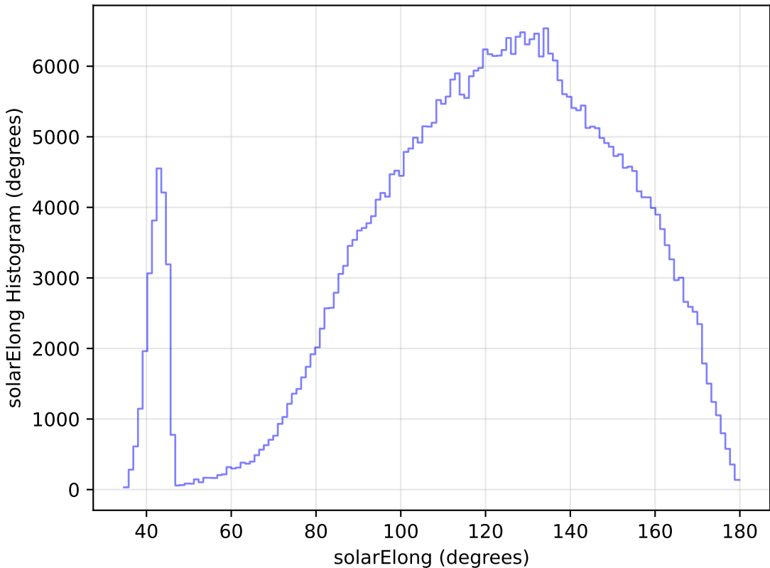
ddf_loaded_half_fl2_v3.4_10yrs All sky z band: solarElong Histogram
