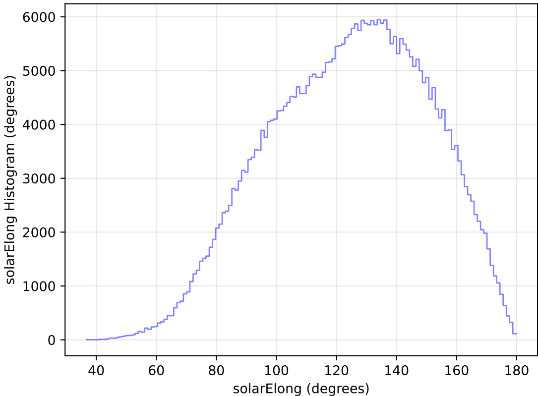
ddf_loaded_half_fl2_v3.4_10yrs All sky y band: solarElong Histogram
