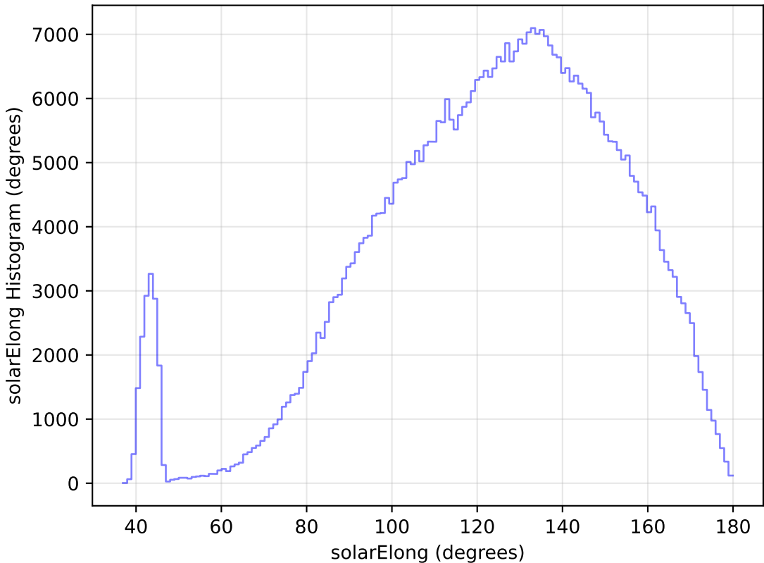
ddf_loaded_half_fl2_v3.4_10yrs All sky r band: solarElong Histogram
