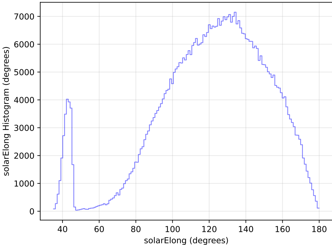
ddf_loaded_half_fl2_v3.4_10yrs All sky i band: solarElong Histogram
