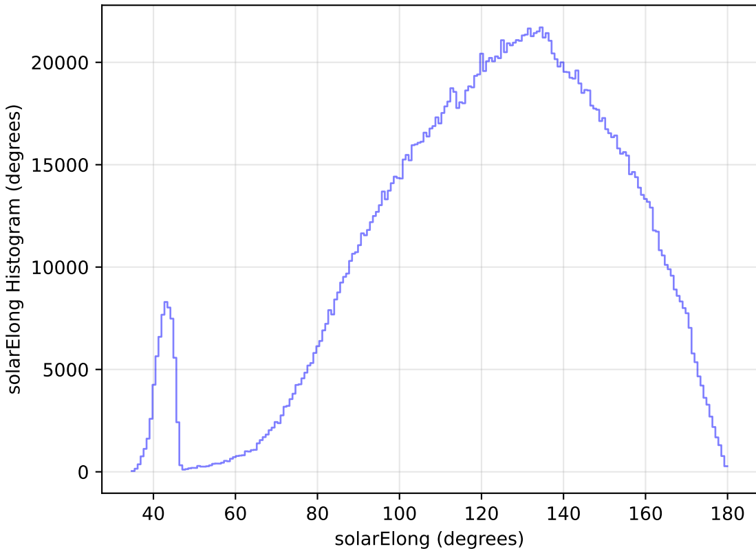
ddf_loaded_half_fl2_v3.4_10yrs All sky all bands: solarElong Histogram
