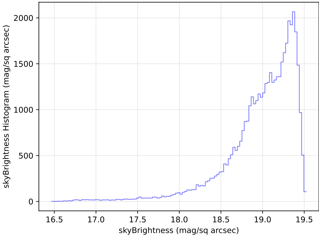
ddf_loaded_half_fl2_v3.4_10yrs Yr 1 z band: skyBrightness Histogram
