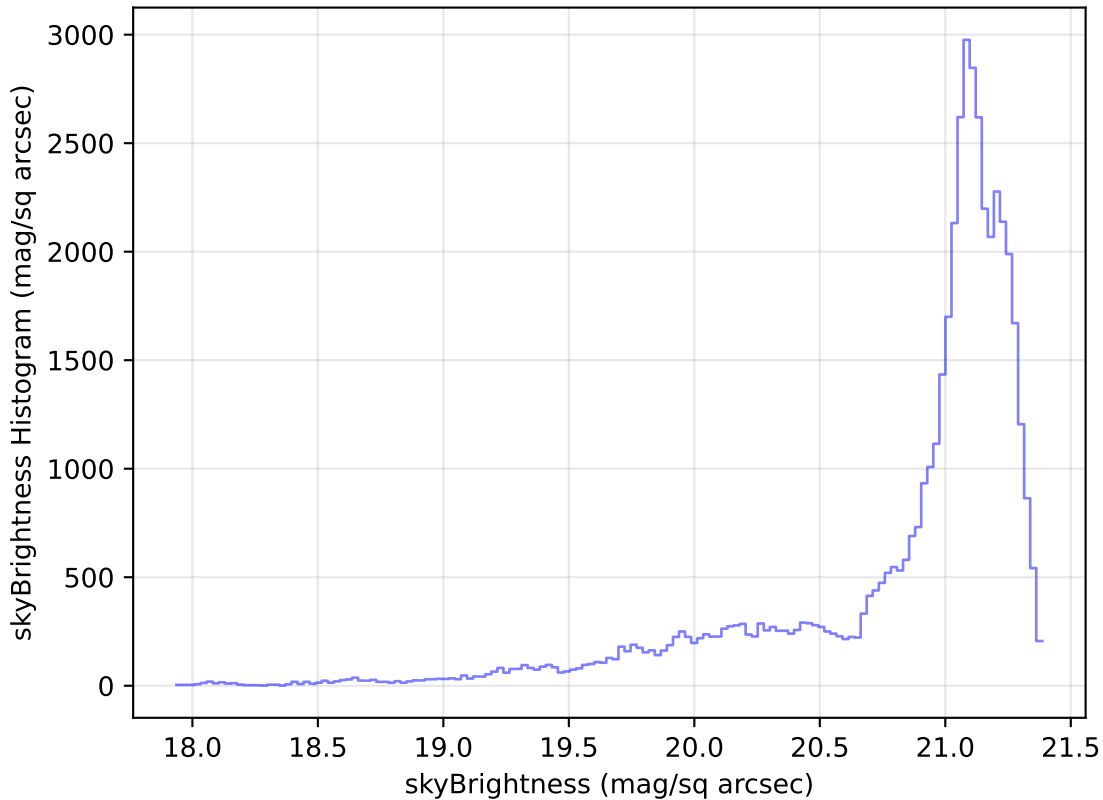
ddf_loaded_half_fl2_v3.4_10yrs Yr 1 r band: skyBrightness Histogram
