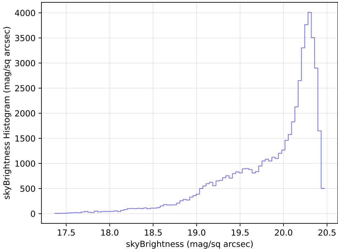
ddf_loaded_half_fl2_v3.4_10yrs Yr 1 i band: skyBrightness Histogram
