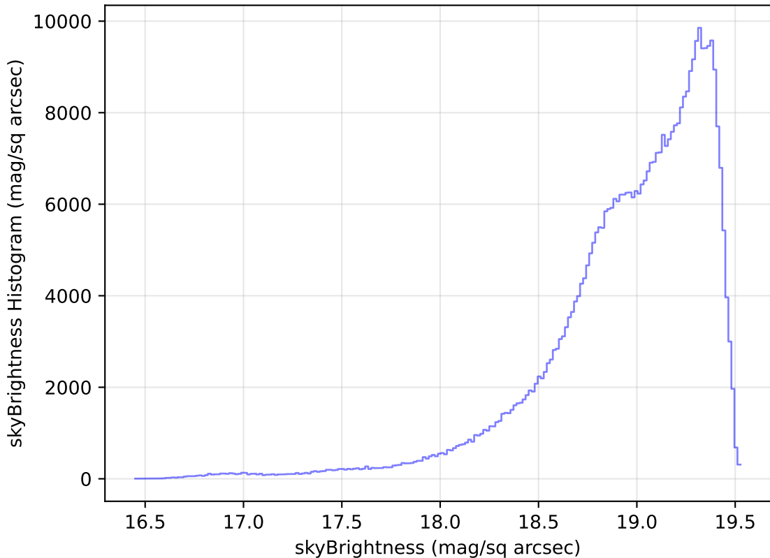
ddf_loaded_half_fl2_v3.4_10yrs WFD z band: skyBrightness Histogram
