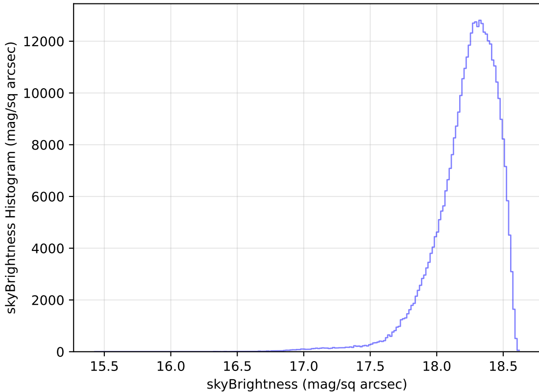
ddf_loaded_half_fl2_v3.4_10yrs WFD y band: skyBrightness Histogram
