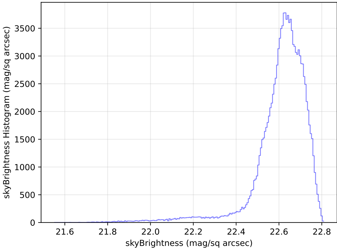
ddf_loaded_half_fl2_v3.4_10yrs WFD u band: skyBrightness Histogram
