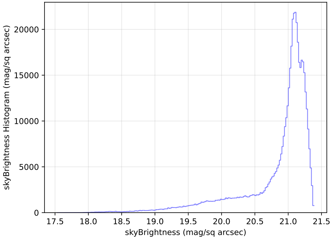
ddf_loaded_half_fl2_v3.4_10yrs WFD r band: skyBrightness Histogram
