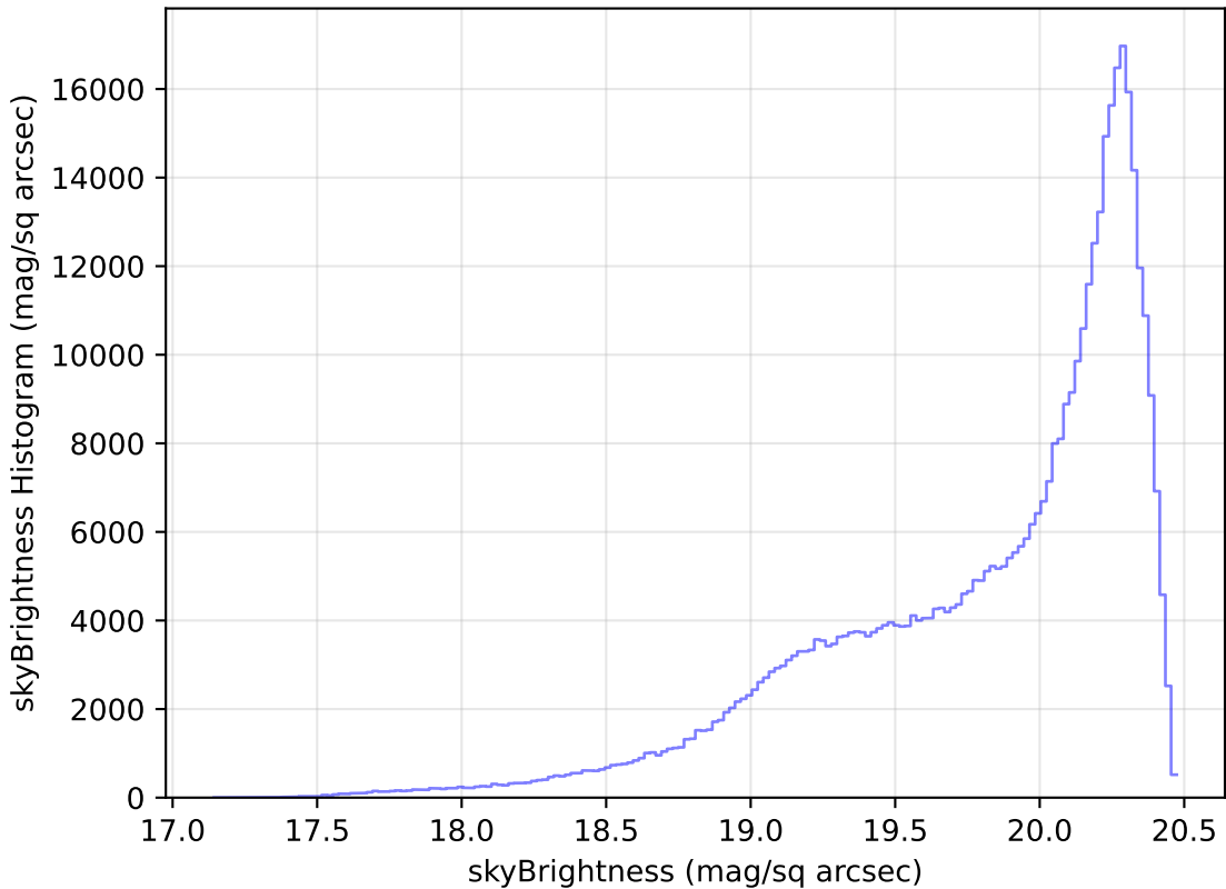
ddf_loaded_half_fl2_v3.4_10yrs WFD i band: skyBrightness Histogram
