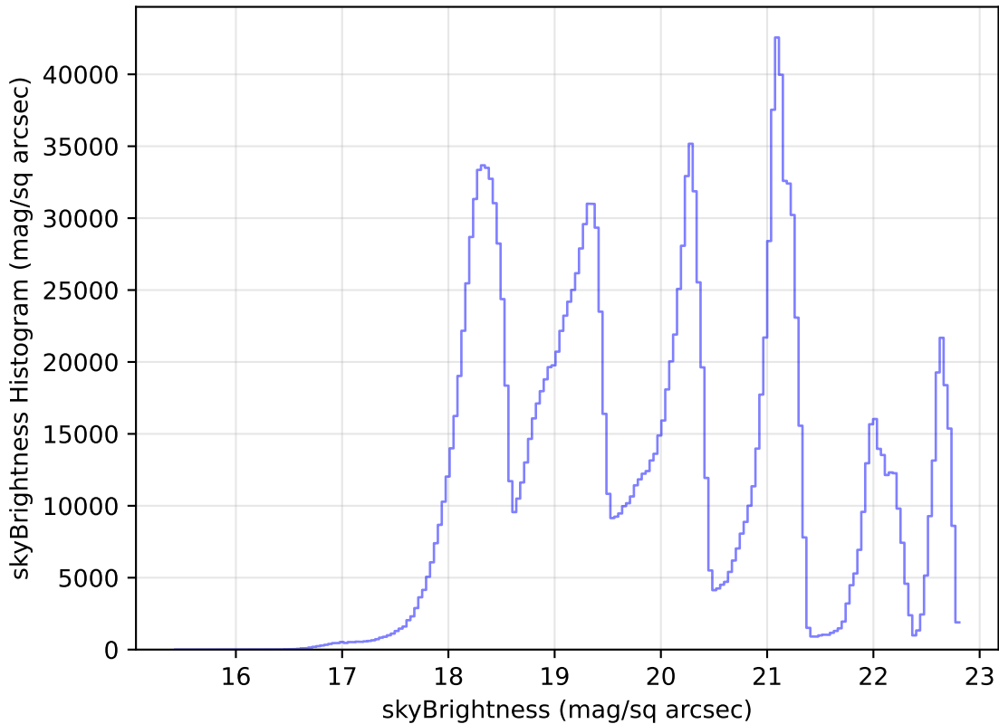
ddf_loaded_half_fl2_v3.4_10yrs WFD all bands: skyBrightness Histogram
