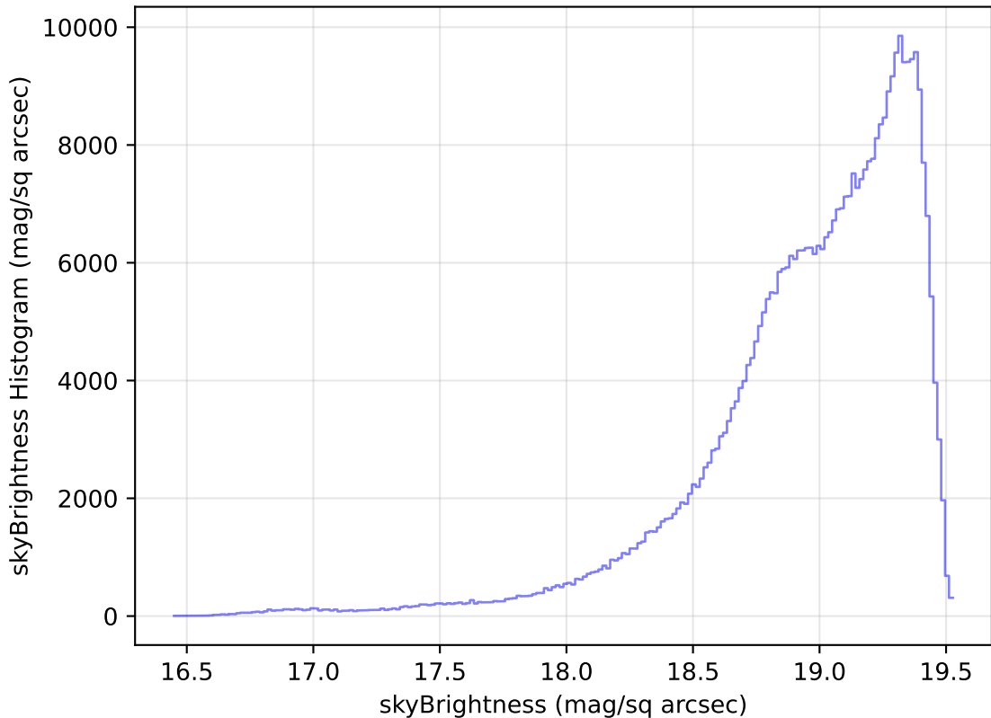
ddf_loaded_half_fl2_v3.4_10yrs All sky z band: skyBrightness Histogram
