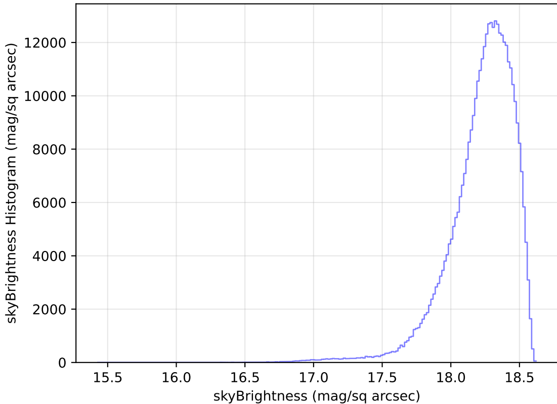
ddf_loaded_half_fl2_v3.4_10yrs All sky y band: skyBrightness Histogram
