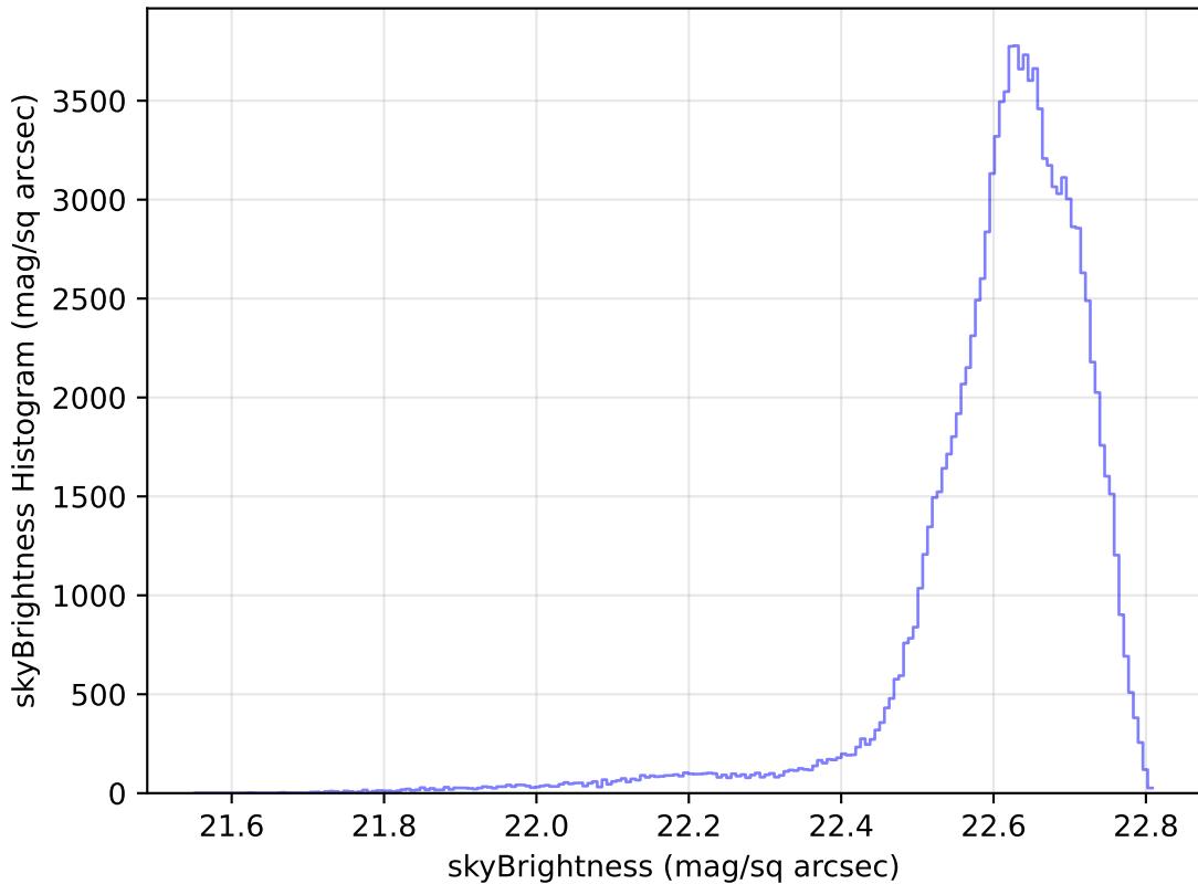
ddf_loaded_half_fl2_v3.4_10yrs All sky u band: skyBrightness Histogram
