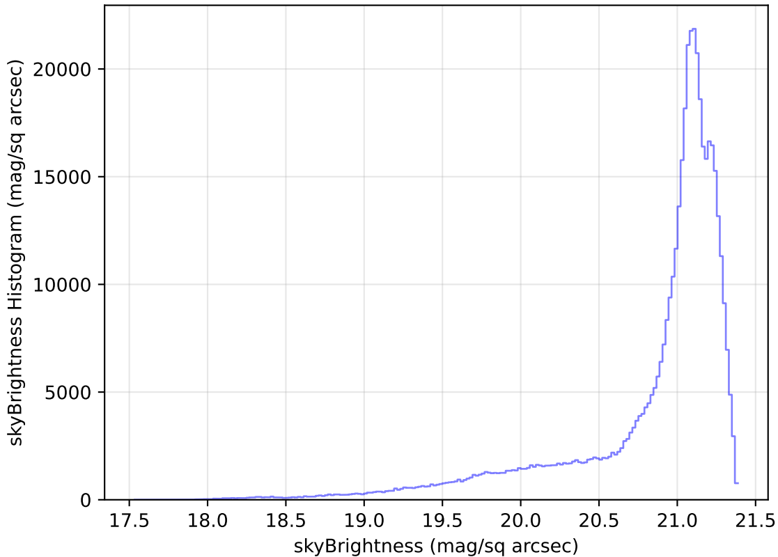
ddf_loaded_half_fl2_v3.4_10yrs All sky r band: skyBrightness Histogram
