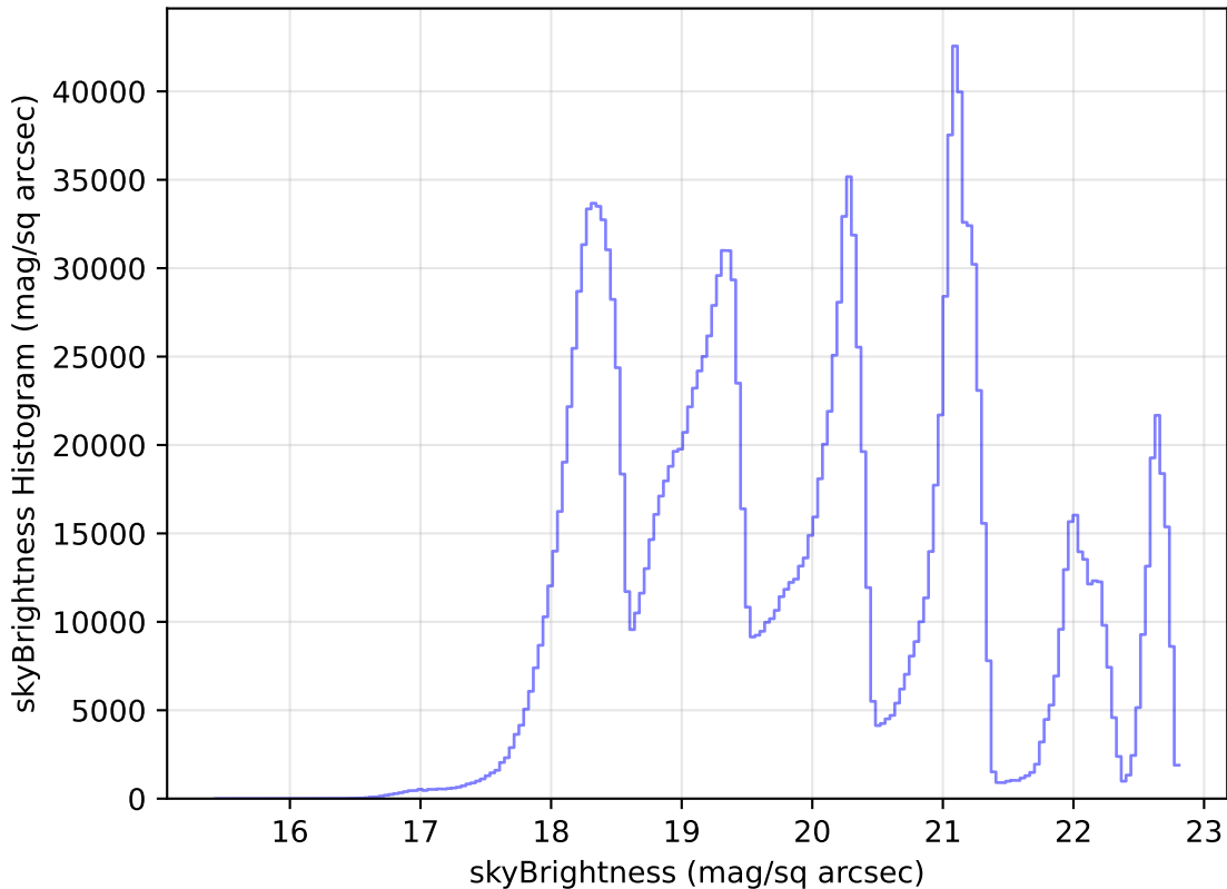
ddf_loaded_half_fl2_v3.4_10yrs All sky all bands: skyBrightness Histogram
