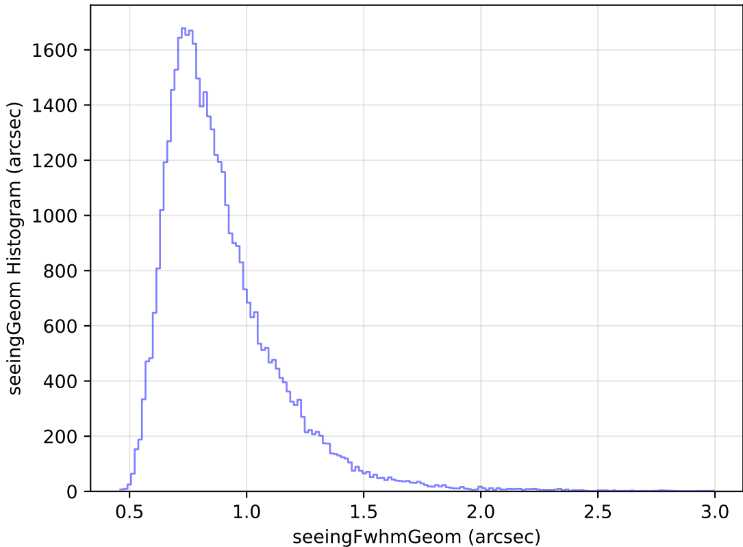
ddf_loaded_half_fl2_v3.4_10yrs Yr 1 z band: seeingGeom Histogram
