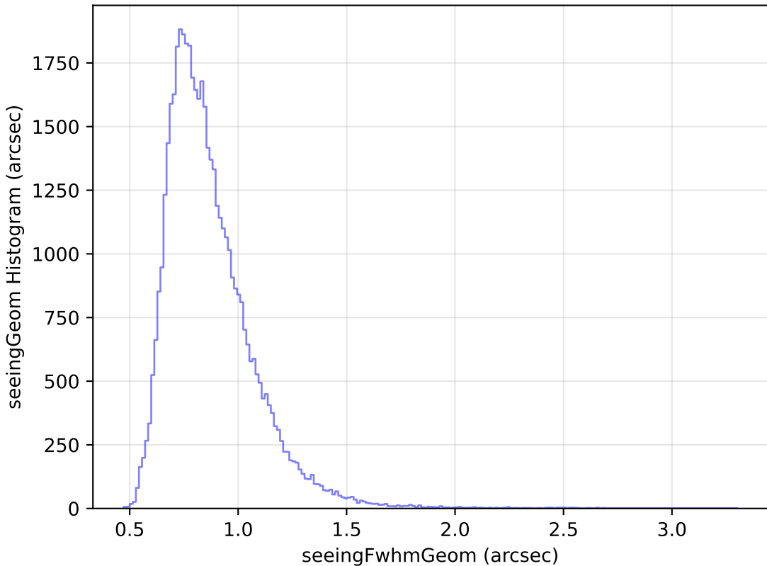
ddf_loaded_half_fl2_v3.4_10yrs Yr 1 y band: seeingGeom Histogram
