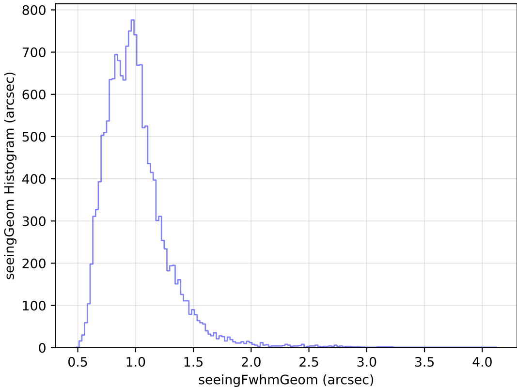
ddf_loaded_half_fl2_v3.4_10yrs Yr 1 u band: seeingGeom Histogram
