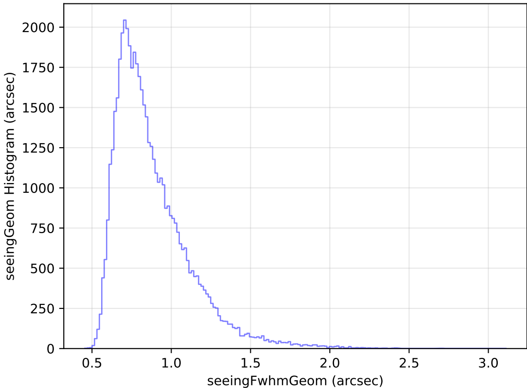
ddf_loaded_half_fl2_v3.4_10yrs Yr 1 r band: seeingGeom Histogram
