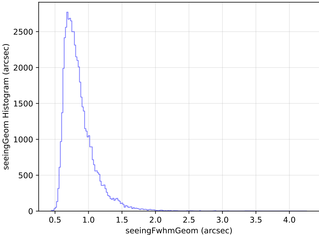
ddf_loaded_half_fl2_v3.4_10yrs Yr 1 i band: seeingGeom Histogram
